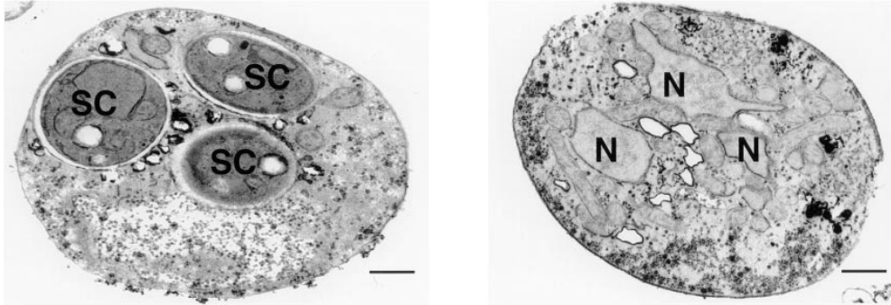
Figure 6. Electron microscopy of sporulated SPO14/SPO14 (NH144) and spo14/spo14 (Y433) cells. (A) A typical wild-type cell late in sporulation (12 h) showing three spore-like compartments. (B) A typical spo14 cell at the same time showing three nuclei but no compartmentalization. SC, spore compartment; N, nucleus. Bars, 500 nm.
