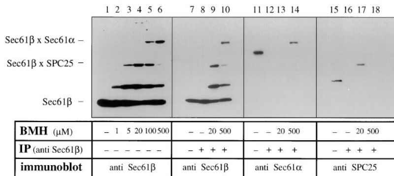
Figure 3. Analysis of the environment of Sec61 \beta by chemical cross-linking. RM were treated with increasing amounts of bis-maleimido-hexane (BMH) and were subsequently analyzed by SDS-PAGE and immunoblotting using antibodies directed against the \beta subunit of the Sec61 complex (lanes 1–6). To identify the cross-linked polypeptides, RM were treated with BMH as indicated. The samples were subsequently immunoprecipitated under denaturing conditions with an anti-Sec61 \beta column. The precipitated material was analyzed by Western blotting using antibodies directed against Sec61 \beta (lanes 7–10), Sec61 \alpha (lanes 11–14) or the 25-kD subunit of the signal peptidase complex (SPC25) (lanes 15–18), respectively. Lanes 1, 7, 11, and 15 show the results for untreated RM.
