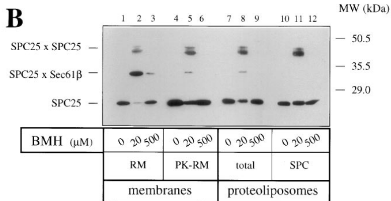
Figure 4. Sec61 \beta is involved in ribosome-dependent structural changes of the translocation site. Rough microsomes (RM), ribosome-free membranes (PK-RM), proteoliposomes produced from an unfractionated detergent extract of PK-RM ( total ), and proteoliposomes containing the purified Sec61 complex ( Sec61p ) or the purified signal peptidase complex ( SPC ), respectively, were treated with BMH as indicated. After SDS-PAGE the samples were analyzed by immunoblotting with antibodies against Sec61 \beta (A) or SPC25 (B). The position of a probable cross-link between Sec61 \beta and Sec61 \gamma is marked by an asterisk .
