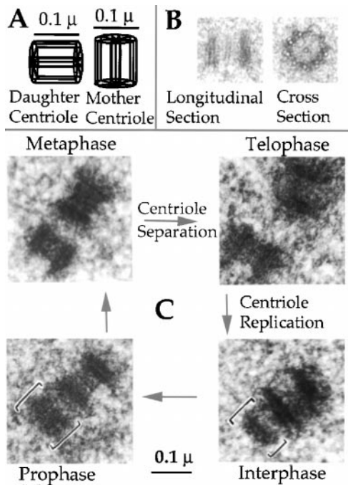
Figure 1. Centriole duplication cycle. (A) A schematic of Drosophila centrioles, which are 105 nm in diameter (measured as the distance between the complete inner tubules) and \sim 110 nm in length (measured as the length of the tubules), and separated by a distance of 46–58 nm. (B) EM longitudinal and cross-sectioned centrioles obtained from high pressure frozen Drosophila embryos. Note that the strongly staining aspect of a centriole in longitudinal thin section appears as parallel lines representing the opposite sides of the cylindrical centriole. (C) The centriole pair undergoes discrete transitions during the cell cycle. Mother and daughter centrioles disengage and move apart as cells exit metaphase. Centriole appearance of a procentriole coincides with entry into S phase, and this daughter (brackets) is complete upon entry into mitosis.
