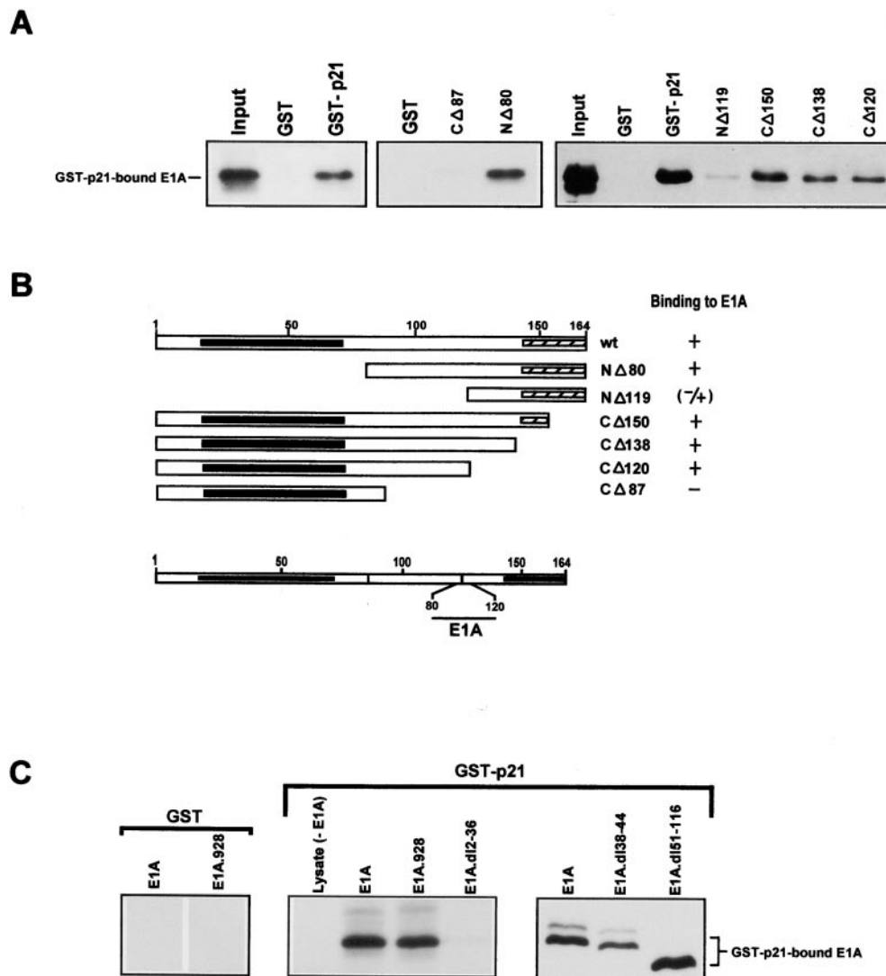
Figure 4. E1A binds directly to p21. (A) GST, GST-p21, or GST-21 deletion mutants, immobilized on glutathione beads, were incubated with purified E1A (75 ng). After elution of the beads, E1A was detected by immunoblot analysis using the anti-E1A mAb M73. Input refers to 100% of the protein used in the binding assay. (B) Schematic representation of p21 and p21 deletion mutants, a summary of their binding activity to E1A, and an illustration of the putative region of p21 to which E1A may interact. The solid box within the p21 drawings represent the binding motifs for cyclin and cdk2. The binding motif for PCNA, as well as a second cyclin binding motif, are shown as hatched boxes. (C) [ 35 S]methionine-labeled wild-type or mutant E1As were produced by in vitro transcription/translation and then mixed with GST-p21 or unfused GST. Complexes after glutathione-Sepharose affinity chromatography were analyzed by SDS-polyacrylamide gels and fluorography.
