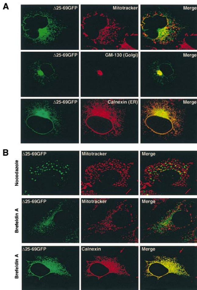
Figure 4. The rTom20-GFP constructs that are incompetent for mitochondria-targeting localized to the ER-Golgi compartments. (A) Localization of \Delta 25 -69GFP to the ER-Golgi compartments. COS-7 cells expressing \Delta 25 -69GFP were immunostained with IgGs against GM130 (Golgi marker) or Calnexin (ER marker). Fluorescent images of GFP (green), GM130 (red), and Calnexin (red) were taken by a confocal microscope. (B) Effect of nocodazole or brefeldin A (BFA) on intracellular localization of \Delta 25 -69GFP. \Delta 25 -69GFP-expressing COS-7 cells were treated with 20 \mu\text{g/ml} nocodazole for 2 h or with 5 \mu\text{g/ml} BFA for 1 h. The cells were then stained with MitoTracker. In a different experiment, \Delta 25 -69GFP-expressing COS-7 cells were treated with BFA as described above, and then immunostained with IgGs against Calnexin (red).
