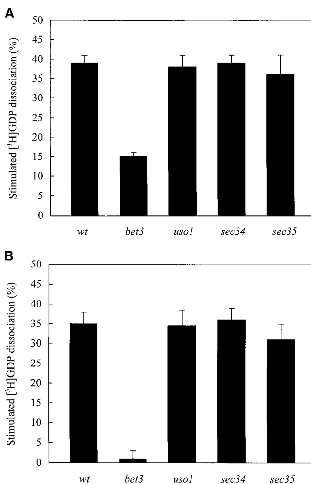
Figure 2. [ 3 H]GDP release from Ypt1p in the presence of cell lysates prepared from ts mutants that block vesicle tethering. His 6 -Ypt1p preloaded with [ 3 H]GDP was incubated with cell lysates for 10 min at 30°C (A) or 37°C (B) as described in the Materials and Methods. Lysates assayed at 37°C were pre-incubated for 5 min at 37°C immediately before the reaction was performed. The amount of [ 3 H]GDP bound to His 6 -Ypt1p was measured using a filter binding assay (Jones et al., 1998). The data are expressed as the percent of radioactivity released from Ypt1p relative to the amount bound before the incubation. The average intrinsic rate of [ 3 H]GDP release from Ypt1p was measured in the presence of BSA (4 mg/ml) and the value obtained (13.0 ± 2% at 30°C; 26.7 ± 4% at 37°C) was subtracted as background. The numbers reported are the average of three separate experiments.
