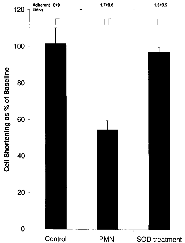
Figure 5. Unloaded cell shortening for control (no PMNs, n = 4 ), PMNs (PMN only, n = 4 ), and SOD treatment (PMN + SOD 300 U/ml, n = 3 ) at 5 min. +, P < 0.05 between indicated groups.
