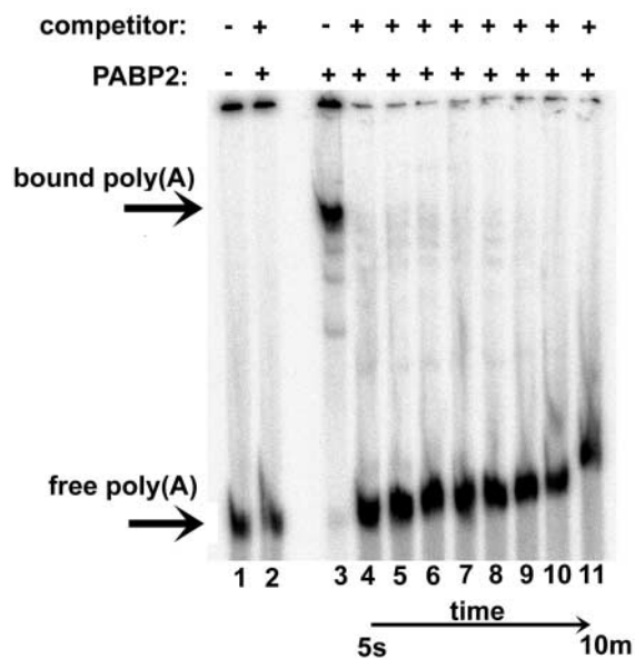
Figure 9. Binding of PABP2 to poly(A) in vitro does not require energy. Binding of PABP2 to oligo ( A_{250} ) was analyzed by an electrophoretic mobility shift assay. PABP2 (10 nM) was incubated at 37°C with ^{32}\text{P} -labeled A_{250} for 30 min and further incubated with 10 \mu\text{M} unlabeled oligonucleotide for the indicated time periods, in the absence of ATP or any other source of energy. Samples were placed while the gel was running.
