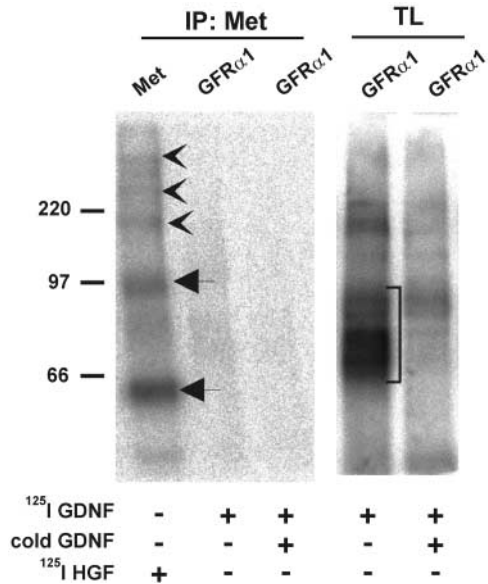
Figure 5. GFR \alpha 1 does not complex with Met. Binding of ^{125} I-GDNF to COS7 cells transfected with gfra1 and ^{125} I-HGF to wild-type COS7 cells followed by cross-linking with EDC together with sulfo-NHS. Immunoprecipitates with anti-Met antibodies (IP:Met) were analyzed by SDS-PAGE under reducing conditions. In total lysates (TL), different complexes of ^{125} I-GDNF (monomers or dimers) and the dimers of GFR \alpha 1 are marked with a square bracket. ^{125} I-HGF \alpha subunit and proHGF are marked by arrows. ^{125} I-HGF-Met complexes are indicated by arrowheads. The results are representative of five independent experiments.
