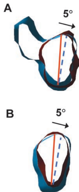
Figure 5. The Unc104 catalytic core rotates by \sim 5^\circ during the ATPase cycle. Thin slices of the catalytic cores of (A) Unc104 446 and (B) Unc104 362 in the AMPPNP (red) and ADP (blue) maps superimposed to show the small \sim 5^\circ rotation between these two nucleotide states. Solid red and dotted blue lines indicate the approximate orientation of the long axes of the catalytic core in the two states. The arrows indicate the rotational relationship between the Unc104 catalytic cores in the two nucleotide states.
