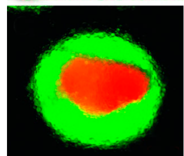
Tension helps sort (top to bottom) ectoderm (red) and mesoderm (green) cells into ordered layers in vitro.
