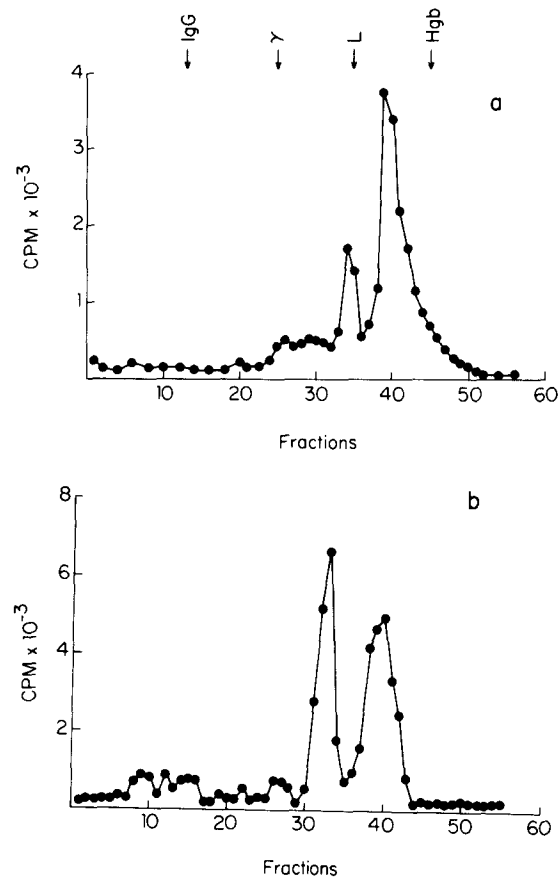
FIG. 2. SDS-acrylamide gel electrophoresis of ^{125}\text{I} -labeled surface proteins binding Con A-arm-Sepharese. (a) Eluted by 0.2 M mannose; and (b) specific serological precipitates with rabbit anti-Con A.
