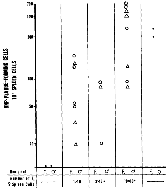
FIG. 2. The number of DNP-PFC/ 10^6 spleen cells in CN \times DN F 1 males which were given different numbers of CN \times DN F 1 female spleen cells which had been previously treated with anti- \theta and C ( \Delta ), or NMS and C ( \circ ). The response to DNP-lys-Ficoll was measured on the 6th day after the administration of the female cells and 100 \mu g of the antigen.
