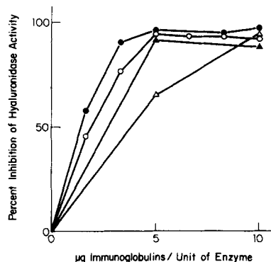
FIG. 3. Inhibition of homologous bound and free hyaluronidase activity by antibody to the purified bound enzyme and by antibody to the whole phage. Purified bound enzymes (1.0 U) obtained from the temperate phage from type 49 streptococcus (strain GT-8760) was incubated with immunoglobulin preparations obtained after gel filtration of antisera against homologous purified bound enzyme (●) or against homologous purified whole phage (△). A phage-free supernate of a mitomycin C-induced lysate of strain GT-8760 containing homologous free enzyme (1.0 U) was incubated with immunoglobulins from antisera against homologous purified bound enzyme (▲) or against homologous purified whole phage (○). After centrifugation to remove immunoprecipitates, residual (unneutralized) enzyme activity was measured on the supernates and the percent inhibition of enzyme activity was calculated (Materials and Methods).
