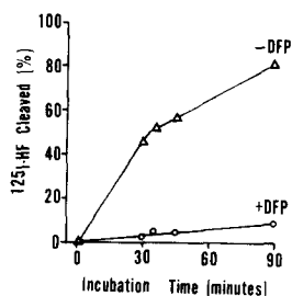
FIG. 3. The rate of proteolytic cleavage of kaolin-bound diisopropylfluorophosphate (DFP)-treated HF incubated in the presence (O) and absence (Δ) of 5 mM DFP.
