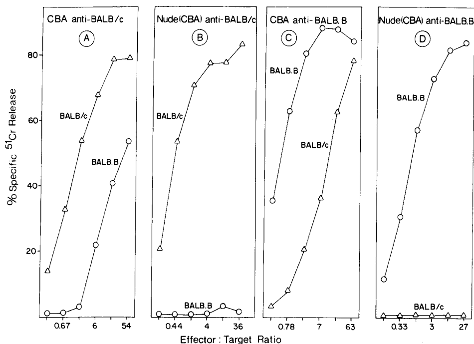
FIG. 4. Lack of cross-reactivity in alloreactive CTL populations from nude mice. Spleen and lymph node cells from a normal (A and C) and a nu/nu (B and D) CBA mouse were stimulated with BALB/c (A and B) or with BALB.B (C and D) spleen cells for two cycles of MLC in the presence of 20% CASUP, and assayed on day 5 of secondary MLC against the following 51 Cr-labeled Con A blasts: BALB/c ( \Delta , spontaneous release 19.7%), and BALB.B ( \circ , spontaneous release 25.6%).
