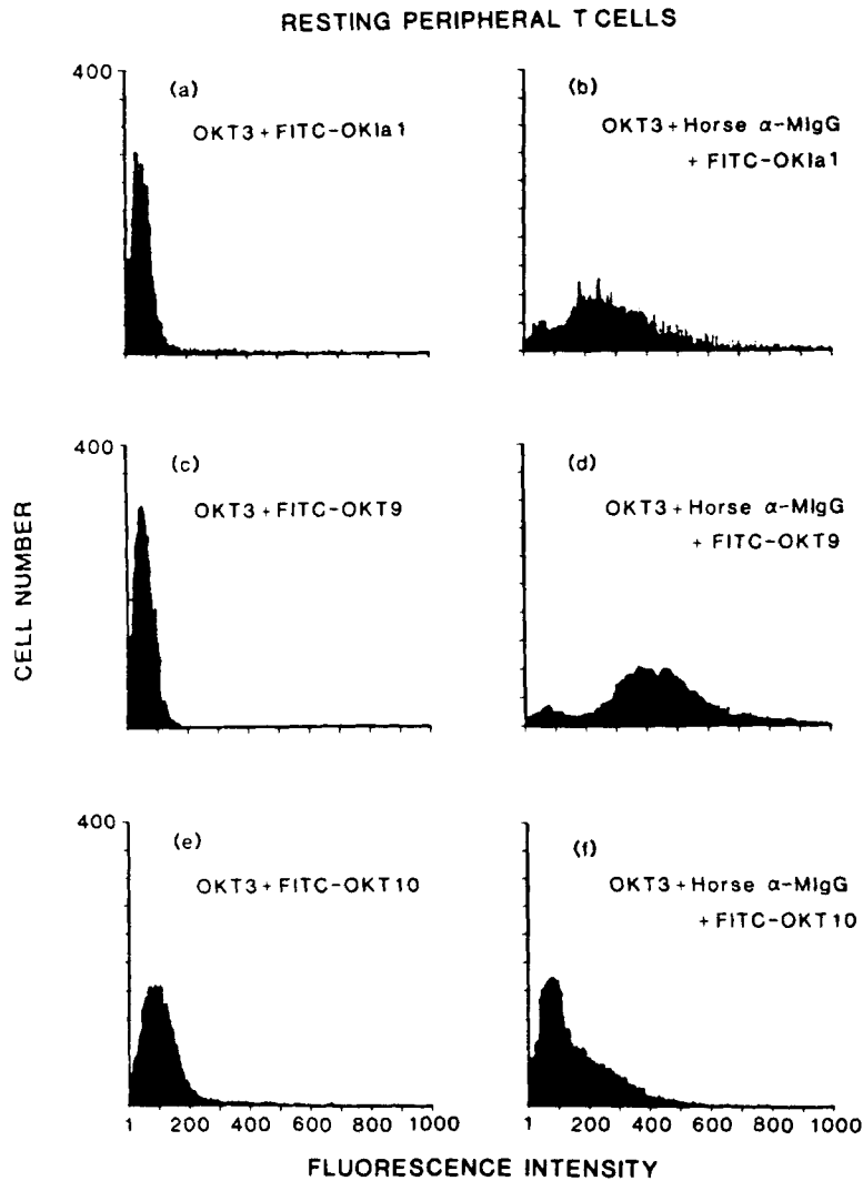
FIGURE 1. Fluorescence histograms of the distribution of activation antigens on resting peripheral T cells following membrane perturbation by cross-linking with OKT3 and horse \alpha -mouse IgG. Cells were treated with: (a) OKT3 + FITC-OKIa1; (b) OKT3 + horse \alpha -mouse IgG and FITC-OKIa1; (c) OKT3 + FITC-OKT9; (d) OKT3 + horse \alpha -mouse IgG and FITC-OKT9; (e) OKT3 + FITC-OKT10; (f) OKT3 + horse \alpha -mouse IgG and FITC-OKT10. The intensity of staining with FITC-OKIa1, FITC-OKT9, and FITC-OKT10 increased when the cells were pretreated with OKT3 and horse \alpha -mouse IgG.
