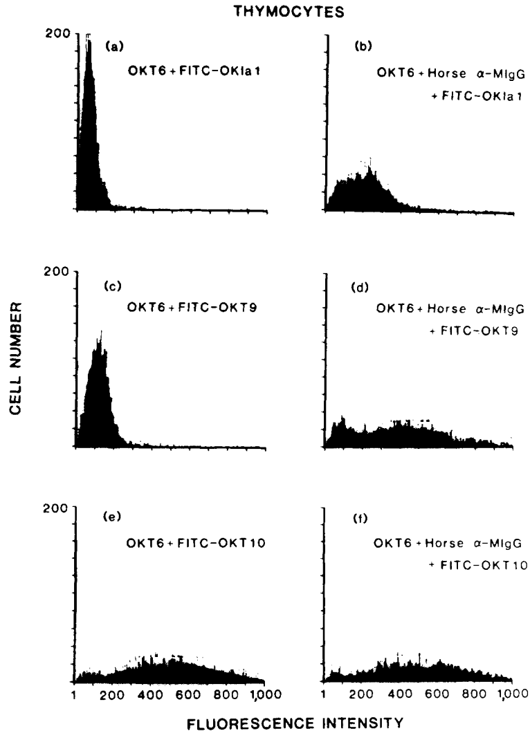
FIGURE 5. Fluorescence histograms of the distribution of activation antigens on thymocytes following membrane perturbation by cross-linking with OKT6 and horse \alpha -mouse immunoglobulin. Cells were treated with: (a) OKT6 + FITC-OKIa1; (b) OKT6 + horse \alpha -mouse IgG and FITC-OKIa1; (c) OKT6 + FITC-OKT9; (d) OKT6 + horse \alpha -mouse IgG and FITC-OKT9; (e) OKT6 + FITC-OKT10; (f) OKT6 + horse \alpha -mouse IgG and FITC-OKT10. The staining intensity of OKIa1 and OKT9 increased when the cells were treated with OKT6 and horse \alpha -mouse IgG before FITC-OKIa1 or FITC-OKT9, whereas the fluorescence staining intensity with OKT10 was high initially and remained unchanged.
