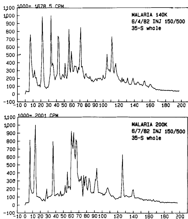
FIGURE 2. Reverse phase chromatography of L 35 S]methionine-labeled peptides of the 200 and 140 K polypeptides digested with TPCK trypsin. [ 35 S]methionine cpm are indicated on the ordinate axis (correction factor noted on top). Tube numbers are indicated on the abscissa.
