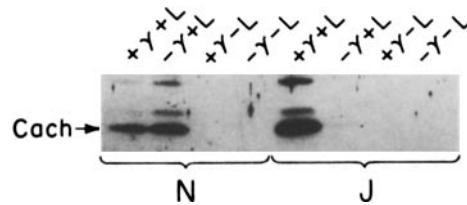
FIGURE 1. Production of cachectin ( Cach ) by peritoneal macrophages obtained from C3H/HeN ( N ) and C3H/HeJ ( J ) mice. Cells were treated with (+) or without (-) endotoxin ( L ) or IFN- \gamma ( \gamma ), each at a concentration of 1 \mu g/ml. Medium was harvested after 16 h and analyzed by immunoconcentration and immunoblotting.
