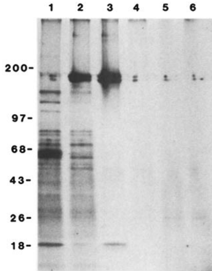
FIGURE 5. SDS-PAGE of Giardia metabolically labeled with [ ^{35}\text{S} ]cysteine. (1) clone of WB A6-6E7R (antigenic variant), (2) WB A6-6E7S (CRP170-expressing); (3) WB A6-6E7S immunoprecipitated with mAb 6E7; (4) WB A6-6E7S immunoprecipitated with control ascites; (5) WB A6-6E7R immunoprecipitated with mAb 6E7; (6) WB A6-6E7R immunoprecipitated with control ascites. Molecular weight markers ( \times 10^{-3} ) are on the left. Note that artifact is present at 170 \times 10^{-3} mol wt marker on lanes 1 and 4-6 due to spillover from lanes 2 and 3.
