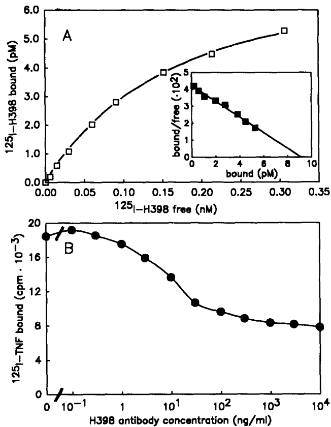
Figure 2. Saturation binding of ^{125}\text{I} -H398 on HL-60 cells and partial competition of H398 with ^{125}\text{I} -TNF binding. (A) Specific ^{125}\text{I} -H398 binding of HL-60 cells was determined as described in Material and Methods. The apparent dissociation constant of H398 binding ( K_d = 2.5 \times 10^{-10} M) and the number of H398 epitopes (1,556/cell) were calculated from Scatchard analyses (see inset). (B) 10^6 HL-60 cells were incubated in duplicates with 20 ng/ml ^{125}\text{I} -TNF and the indicated concentrations of H398 antibody for 3 h at 0^\circ\text{C} . Nonspecific binding in the presence of a 200-fold excess of unlabeled TNF was 2,150 cpm and is subtracted in the graph.
