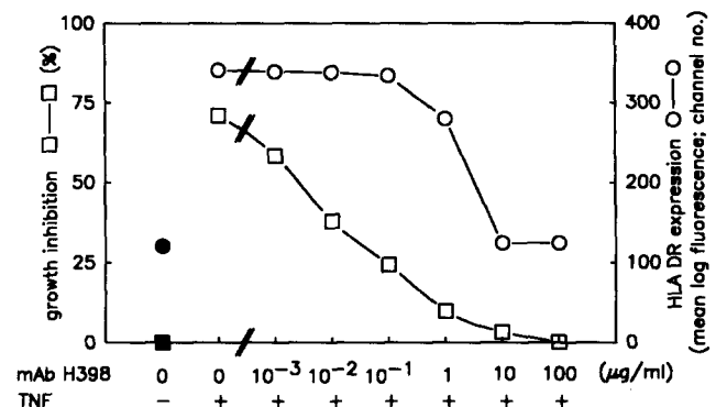
Figure 4. H398 antibody is a TNF antagonist. Shown is the dose-dependent inhibition of TNF-mediated cytoxicity on U937 cells ( \square ) (left axis) and of TNF-mediated enhancement of HLA-DR expression in Colo 205 cells ( \circ ) (right axis). In both assay systems, the presence of IFN- \gamma is required to induce the respective TNF responses (18, 27, 28). Modulation of TNF cytostatic activity on U937 cells is given in percent growth inhibition of IFN- \gamma -treated U937 cells ( \blacksquare ) (8,191 cpm). HLA-DR antigen expression in Colo 205 cells is given in arbitrary fluorescence units on a log scale. Untreated Colo 205 cells are HLA-DR ^- (mean log fluorescence intensity of 54 vs. 52 with control antibody). IFN- \gamma induces gene expression ( \bullet ) (mean log fluorescence intensity of 121), which is enhanced by TNF (27). U937 and Colo 205 cells were cultured for 40 h in the presence of 10 and 0.02 ng/ml of IFN- \gamma , respectively, with or without 1 ng/ml TNF and log _{10} dilutions of H398 antibody. U937 cells were then pulsed with [ ^3\text{H} ]thymidine for 6 h (28). Each value represents the mean of six replicates (SD <18%). Colo 205 cells were analyzed for HLA-DR expression by immunofluorescence flow cytometry.
