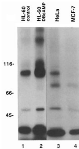
Figure 3. Chemical crosslinking studies with ^{125}\text{I} -TNF on different cell lines reveal two distinct receptor proteins. Membrane-bound ^{125}\text{I} -TNF was crosslinked with disuccinimidyl suberate and analyzed by SDS-PAGE as described in Materials and Methods. Arrows indicate the two major crosslinking products of 100 and 78 kD, respectively.
