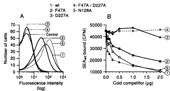
Figure 2. Binding of wild-type and mutated SEA to IFN- \gamma -treated THP1 as detected by flow cytometry (A), and the ability of SEA mutants to inhibit 125 I-labeled wild-type SEA binding to IFN- \gamma -treated THP1 (B). For flow cytometric analysis, cells were first incubated with SEAw t or SEA mutants, followed by anti-SEA mAb. Cells were then washed, rabbit anti-mouse IgG-FITC conjugate was added, and cells were incubated for 30 min. Washed cells were then analyzed by FACScan ® . For binding inhibition assay, cells were incubated with 125 I-labeled SEA in the absence or the presence of cold SEAw t or SEA mutants. Cells were then pelleted through an oil cushion (84% silicon oil and 16% mineral oil), and their activity (cpm) was determined using a gamma counter. All tests were performed in triplicate, and SEM was <10% in all assays.
