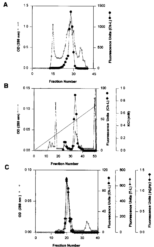
Figure 7. Purification and characterization of T. cruzi proteasomes. (A) Gel filtration on Superose 6. The chymotrypsin activity in fractions 17–24 was totally inhibited by lactacystin but unaffected by E-64. (B) Anion-exchange chromatography of pooled fractions 17–24 on a Mono Q column. Bound proteins were eluted using a 0–1 mM KCl linear gradient. Fractions that displayed Ch-L activity that was inhibitable by lactacystin, but not by E-64, were eluted at approximately 400–500 mM KCl. (C) Gel Filtration on Superose 6. Fractions eluted from the Mono Q at 400–500 mM KCl were loaded onto Superose 6 16/30. Proteolytic activities under the major protein peak were measured with the following fluorogenic peptides: Suc-Leu-Leu-Val-Tyr-MCA for Ch-L activity (Ch-L), Boc-Leu-Arg-Arg-MCA for T-L activity (T-L) and Z-Leu-I.eu-Glu- \beta NA for peptidylglutamyl peptide hydrolase (PGPH). All activities were strongly inhibited by lactacystin but not by E-64.
