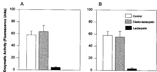
Figure 9. In vivo and in vitro inhibition of T. cruzi proteasomes by lactacystin. (A) Trypomastigotes were incubated for 3 h in transformation medium containing 10 \mu M lactacystin (solid bars), or clasto-lactacystin (striped bars) or with medium alone (open bars). Samples of parasites ( 3 \times 10^7 ) were washed with PBS, resuspended in 200 \mu l of 20 mM Tris, somaticated, and centrifuged. Supernatants were immunoprecipitated with polyclonal antibodies raised against T. cruzi proteasomes. Immunocomplexes were collected using protein A-Sepharose, and the Ch-L activity associated with the beads was measured. When parasites were treated with medium and immunoprecipitated with preimmune serum, no Ch-L activity was detected. (B) As additional controls for the specificity of the immunoprecipitation reaction, untreated parasites were somaticated, treated with lactacystin (solid bars), or clasto-lactacystin (striped bars), or medium (open bars) and immunoprecipitated as above. The Ch-L activity of the immunoprecipitates was then measured. All experiments were performed in triplicate, and results expressed as mean \pm SD.
