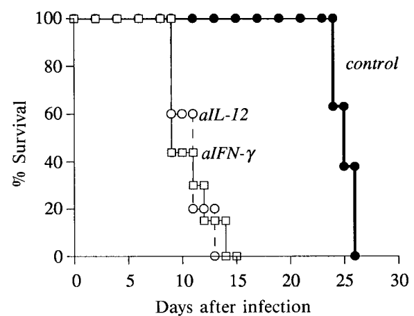
Figure 4. Innate resistance to T. gondii in iNOS ko mice is IL-12- and IFN- \gamma -dependent. iNOS ko animals were injected i.p. with 1 mg of either normal rat IgG ( n = 8 ), anti-IFN- \gamma mAb XMG-6 ( n = 7 ), or anti-IL-12 mAb C17.8 ( n = 5 ) 1 d before infection with 20 cysts. Survival was monitored as in Fig. 1. The experiment shown is representative of three performed.
