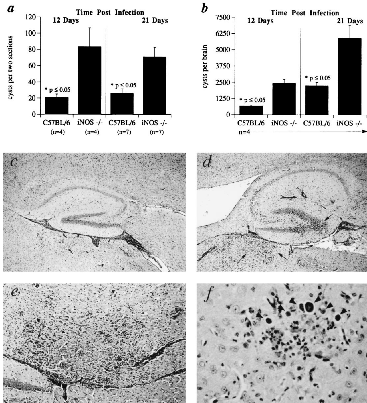
Figure 3. Brains of iNOS ko mice show increased cyst burdens as well as necrotizing encephalitis. C57BL/6 and iNOS ko mice were infected i.p. with 20 cysts each and brains harvested 12 and 21 d later for cyst enumeration in histological sections (A) or tissue homogenates (B). The mean cyst count and SE are shown for each group consisting of the number of animals indicated. (C–F) Photomicrographs of periodic acid–Schiff’s stained, sagittal sections of brains from iNOS (D–F) and C57BL/6 (C) mice at 21 d after infection. Hippocampal regions of the brain in C57BL/6 (C) and iNOS ko (D) mice. Large areas of inflammation and necrosis seen in the iNOS brain (D) but not in C57BL/6 brain (C) are indicated by arrows. E shows a higher magnification of the same necrotizing lesion in D. (F) Brain section from iNOS ko mouse with numerous cysts (arrowheads) arranged in a satellite-like array, a feature frequently observed in these animals. Original magnification: (C and D) \times 50 ; (E) \times 200 ; (F) \times 400 .
