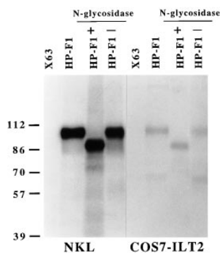
Figure 3. The HP-F1 \gamma receptor is an ~110-kD monomeric glycoprotein. (Left) Immunoprecipitation from 125 I-labeled NKL cells with HP-F1 mAb yields a protein which runs as a 110-kD band in SDS-PAGE under reducing conditions. After treatment with N -glycosidase, the molecular mass is reduced to ~90 kD. (Right) Identical electrophoretic patterns were obtained by SDS-PAGE analysis of immunoprecipitates from ILT2-transfected COS7 cells. No bands were detected using the culture supernatant from X63 murine myeloma in control experiments.
