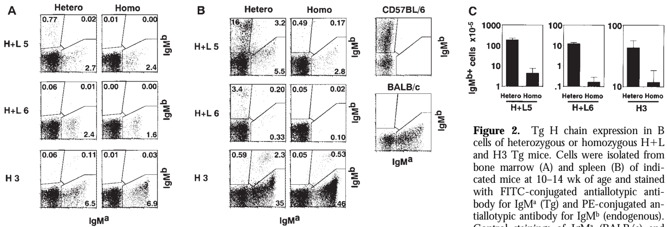
Figure 2. Tg H chain expression in B cells of heterozygous or homozygous H+L and H3 Tg mice. Cells were isolated from bone marrow (A) and spleen (B) of indicated mice at 10–14 wk of age and stained with FITC-conjugated anti-allotypic antibody for IgM a (Tg) and PE-conjugated anti-allotypic antibody for IgM b (endogenous). Control stainings of IgM a (BALB/c) and IgM b (C57BL/6) spleen cells are shown. The percentages of cells of each gated region in total viable cells are indicated. Total numbers of the cells with endogenous H chains in heterozygous or homozygous H+L5, H+L6, and H3 Tg mice are shown (C). Spleen cells were stained and analyzed from at least three mice of each Tg line. Numbers of indicated cells were calculated by (percentage of indicated cells in viable cells) × (No. of viable cells). Results are expressed as mean ± SD.
