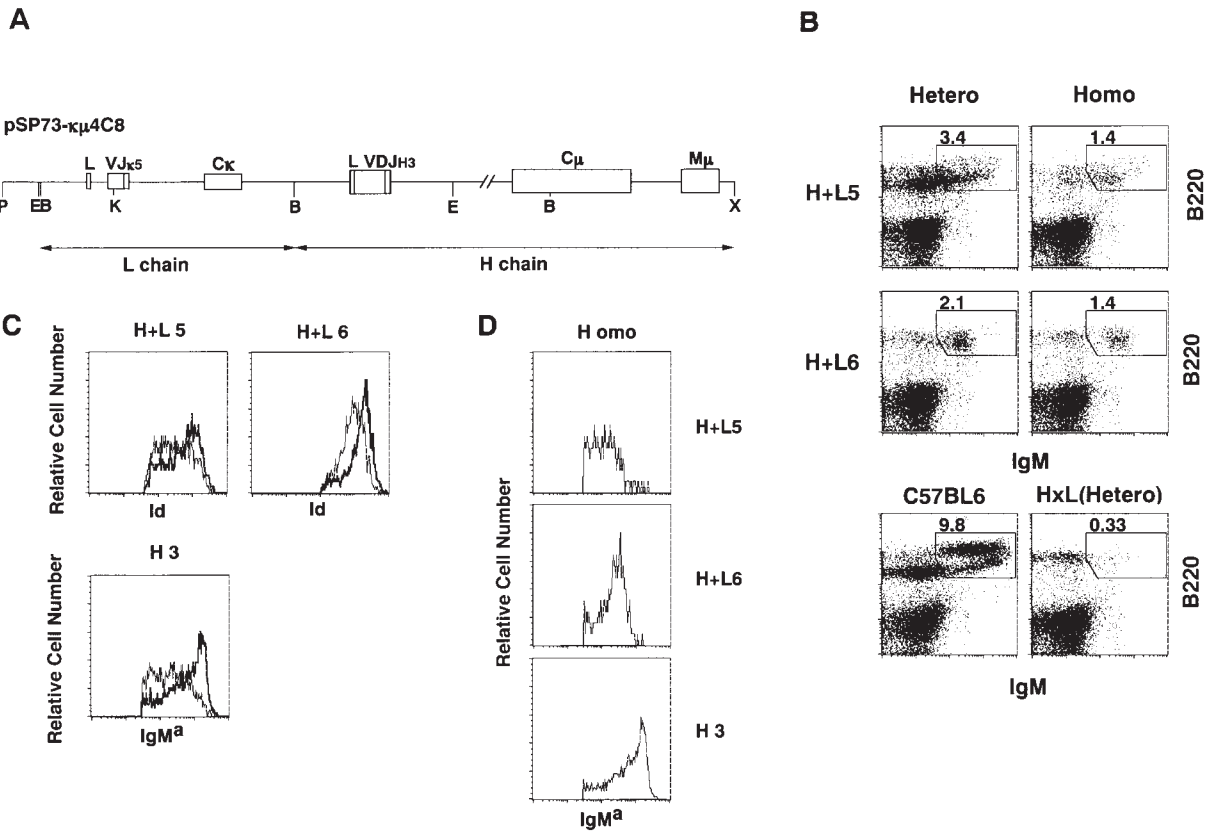
Figure 1. Structure and expression of anti-RBC transgene. (A) Tg construct with tandem joined H and L chain genes. DNA fragments of the L and H chain genes are shown by arrows. Exons are represented by open boxes. Relevant restriction sites are shown: B, BamHI; E, EcoRI; X, XhoI; K, KpnI; P, PvuI. (B) Flow cytometric analysis of bone marrow cells in Tg mice. Bone marrow cells were isolated from heterozygous (hetero) H+L5, homozygous (homo) H+L5, hetero H+L6, homo H+L6, C57BL/6, and HxL mice at 10–14 wk of age and stained with biotin-conjugated goat anti-mouse IgM antibody, followed with FITC-conjugated anti-B220 antibody and Cy-Chrome ® -conjugated SA. The percentages of B220 + IgM + cells of the gated region in the total viable cells are indicated in each panel. (C) Flow cytometric analysis for surface expression of the Tg Ig in heterozygotes and homozygotes. Bone marrow cells were isolated from heterozygous (thin line) or homozygous Tg mice (thick line) of H+L5, H+L6, and H3 mice at 10–14 wk of age. Bone marrow cells were stained with either biotin-conjugated anti-Id antibody (S54) followed by PE-conjugated SA or FITC-conjugated anti-allotypic antibody for IgM a (Tg). (D) Flow cytometric analysis of relative surface Tg expression in homozygous Tg lines. Staining was done as described in panel C using FITC-conjugated anti-IgM a antibody.
