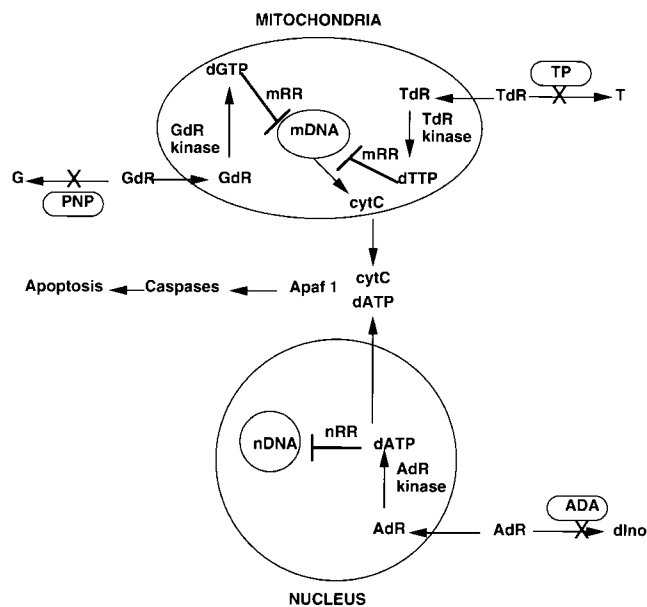
Figure 11. Proposed mechanism of PNP, ADA, and TP deficiencies. Mutations in the cytosolic enzymes PNP and TP result in accumulation of deoxyguanosine (GdR) and thymidine (TdR), respectively. The accumulated deoxynucleosides are phosphorylated by the mitochondrial enzymes deoxyguanosine kinase (GdR kinase; reference 47) or thymidine kinase (TdR kinase; reference 61), resulting in the accumulation of dGTP and dTTP, respectively. The abnormal accumulation of dNTP may interfere with mitochondrial DNA synthesis, or repair directly or by inhibition of mitochondrial ribonucleotide reductase (mRR; reference 62), leading to apoptosis. In contrast, ADA deficiency leads to the accumulation of dATP in the nucleus because of nuclear localization of deoxycytidine kinase, the enzyme responsible for deoxyguanosine phosphorylation (reference 27). Accumulation of dATP leads to apoptosis in a p53-dependent manner by inhibiting nuclear ribonucleotide reductase (nRR), interfering with DNA repair, and by directly participating in caspase activation (references 7, 31, 60).
