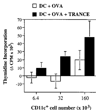
Figure 4. Increased presentation of antigens by DCs from the draining LNs of mice immunized with TRANCE-treated DCs. Immature bone marrow-derived DCs were pulsed for 6 h with or without 10 \mu\text{g}/\text{ml} OVA. The cells were dislodged and transferred to new 100-mm culture dishes for 48 h to allow maturation. During the last 12 h, the cells were pulsed with 1 \mu\text{g}/\text{ml} soluble TRANCE (black bars) or with medium alone (white bars). The DCs were then washed, and 5 \times 10^5 cells were
