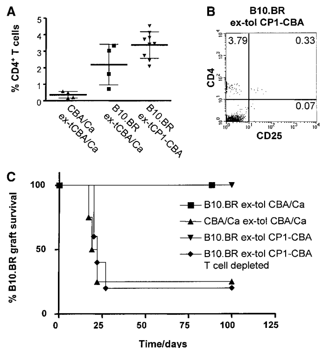
Figure 5. T cells expand from the tolerated B10.BR skin grafts. RAG1^{-/-} -CBA mice were grafted with tolerated B10.BR skin from tolerant CBA/Ca mice (■), CBA/Ca skin from CBA/Ca mice tolerant to B10.BR skin grafts (▲), and tolerated B10.BR skin grafts from tolerant CP1-CBA mice (▼ and ◆). Tolerated B10.BR skin grafts in group ◆ were depleted of putative infiltrating T cells with 0.25 mg CAMPATH-1H at day -1 . (A) Blood samples were collected 30 d after skin grafting and analyzed by FACS ® . The graph represents the percentage of CD4^+ T cells within blood mononuclear cells. The percentage of CD4^+ T cells that expanded from tolerated skin grafts is significantly higher than in the animals grafted with CBA/Ca skin from tolerant syngeneic donors ( P < 0.05 , unpaired t test). (B) FACS ® staining from a mouse of the tolerated skin group (▼), showing that expanded T cells are mainly CD4^+CD25^- . (C) All mice were transfused with 10^7 spleen cells from naive CBA/Ca 1 wk after blood tests, and transplanted with a fresh B10.BR skin on the following day (day 0). Recipients of tolerated B10.BR skin grafts whose putative regulatory T cells had not been depleted resisted the challenge with transfused CBA/Ca splenocytes and accepted the B10.BR skin grafts indefinitely (■ and ▼, MST > 100 d, P < 0.05 ). Mice that were recipients of tolerated B10.BR skin grafts depleted of T cells rejected the grafts shortly after transfusion of CBA/Ca splenocytes (▲, MST = 22 d). Recipients of CBA/Ca skin from CBA/Ca mice tolerated to B10.BR skin grafts also rejected B10.BR skin grafts (◆, MST = 20.5 d).
