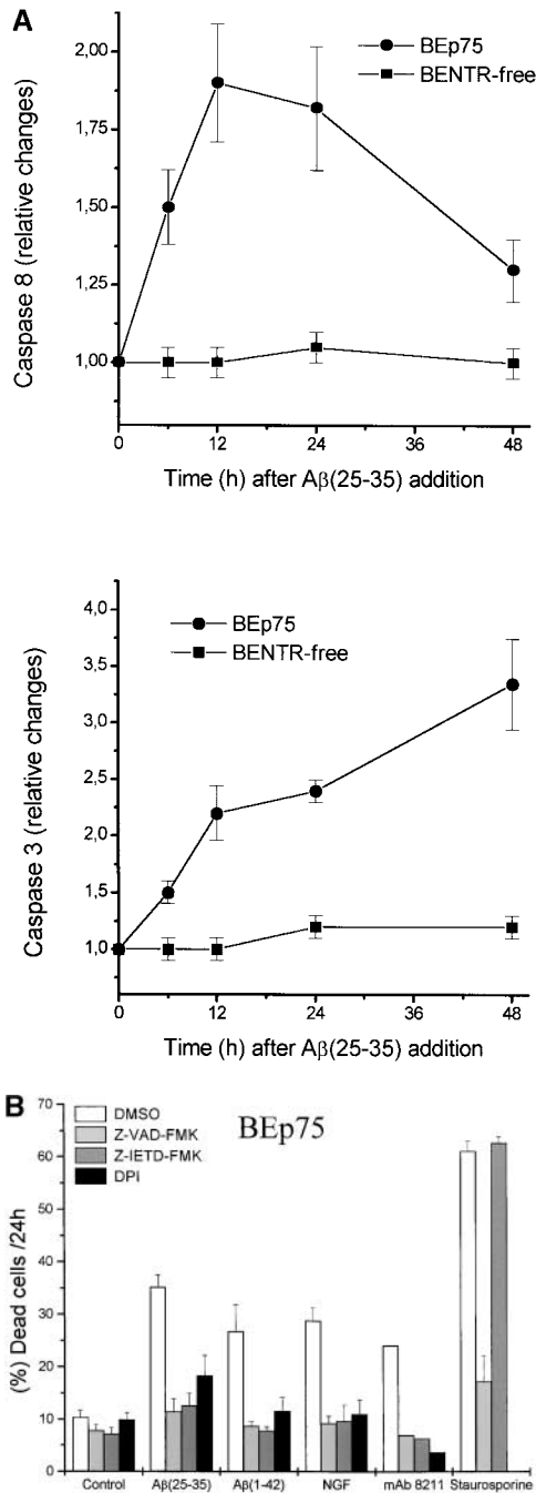
Figure 4. Metabolic features of cell death induced by A \beta . (A) Time course of the activation of caspases-8 and -3 as induced by a treatment with A \beta (25–35) (20 \mu M). Results shown are means \pm SD of four experiments. (B) Effect of Z-VAD-FMK (100 \mu M), a nonspecific inhibitor of caspases, of Z-IETD-FMK (20 \mu M), a specific inhibitor of caspase-8, and of DPI (100 nM), an inhibitor of ROI-forming NADPH oxidase and other flavoprotein dehydrogenases, on the cytotoxic activity by A \beta (25–35) (20 \mu M), A \beta (1–42) (5.0 \mu M), NGF (10 nM), mAb 8211 (5.0 \mu g/ml), and staurosporine (200 nM) in BEp75 cells. Data are reported as means \pm SD of three to four experiments (mAb 8211, two experiments).
