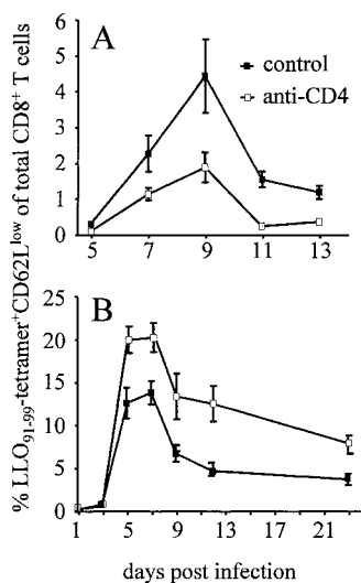
Figure 1. LLO 91-99 -specific CD8 + T cell response during primary and secondary infection with L. monocytogenes (A) Primary infection: mice infected with L. monocytogenes were left untreated (control) or received anti-CD4 mAb (anti-CD4). (B) Secondary infection: mice were infected and after 60 d challenged with L. monocytogenes . During challenge infection, mice were left untreated or received anti-CD4 mAb. At the indicated days, spleen cells were stained with Cy5-conjugated anti-CD8 \alpha mAb, FITC-conjugated anti-CD62L mAb, and PE-labeled LLO 91-99 -tetramers, and analyzed by flow cytometry after the addition of propidium iodide. Figures show percent values of live CD62L low tetramer + cells of total CD8 + cells. Data represent mean \pm SD of three mice per group and time point. Experiments in A and B are representative of two or three experiments, respectively.
