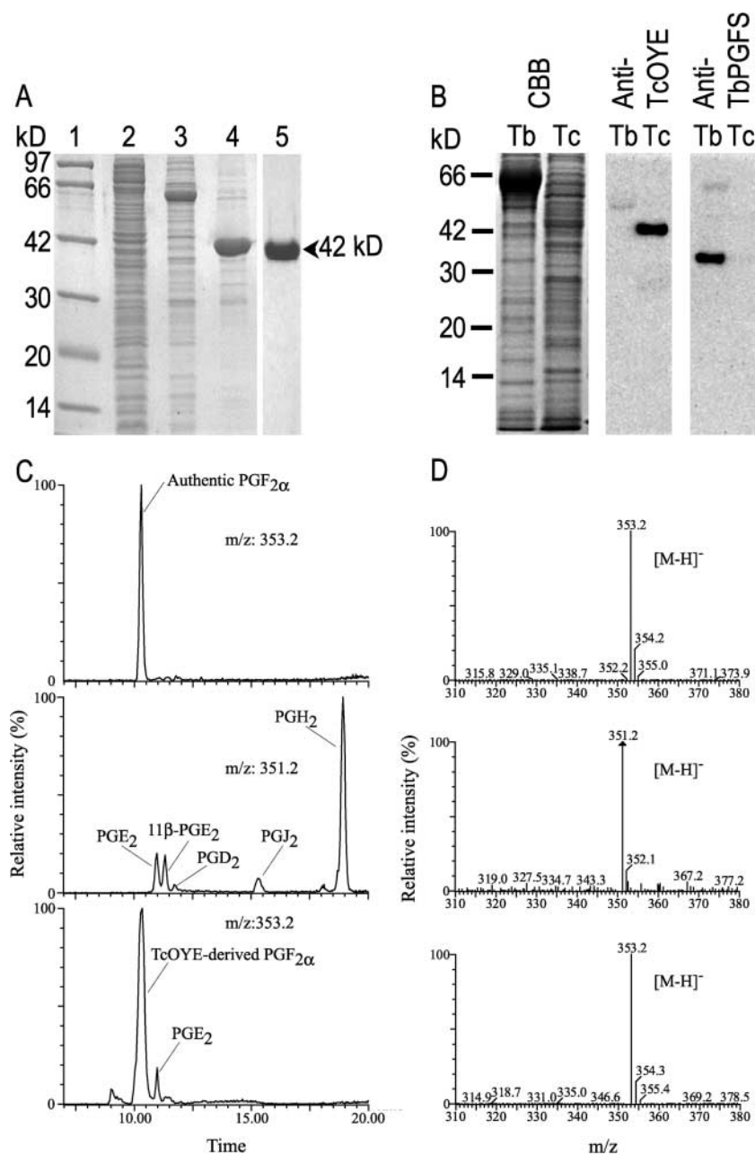
Figure 4. (A) Purification of recombinant TcOYE. TcOYE was expressed as a fusion protein with GSH in E. coli BL21. Lane 1, molecular weight markers; lane 2, lysates from noninduced E. coli BL21 cells expressing pGEX-TcOYE; lane 3, lysates from IPTG-induced E. coli BL21 cells expressing pGEX-TcOYE; lane 4, after affinity chromatography; lane 5, pure recombinant TcOYE. (B) Immunoblot analyses of cell extracts from T. cruzi epimastigote and T. brucei bloodstream form. After blotting, the membranes were incubated with anti-TcOYE or anti-TbPGFS polyclonal antibodies. On the left, SDS-PAGE of the lysates corresponding to T. brucei (Tb) and T. cruzi (Tc) is shown. The proteins were detected with Coomassie Brilliant Blue (CBB). The middle shows a Western blot for proteins incubated with anti-TcOYE polyclonal antibody. The right shows a Western blot for proteins incubated with anti-TbPGFS polyclonal antibody. (C) LC-MS chromatograms of the relative ion intensity for TcOYE-generated PGF 2α . Top, standard PGF 2α ; left, substrate (9,11-endoperoxide PGH 2 ) showing traces of nonenzymatic degradation products (PGE 2 , 11β-PGE 2 , PGD 2 , and PGJ 2 ); bottom, PGF 2α resulting from the reduction of the substrate by TcOYE. The chromatograms for PGE 2 , 11β-PGE 2 , PGD 2 , and PGH 2 were visualized at m/z = 351.2 , whereas that of PGF 2α was monitored at m/z = 353.2 . (D) Mass spectra showing the [M-H] - ions of authentic PGF 2α (top), PGH 2 (middle), and TcOYE-generated PGF 2α (bottom).
