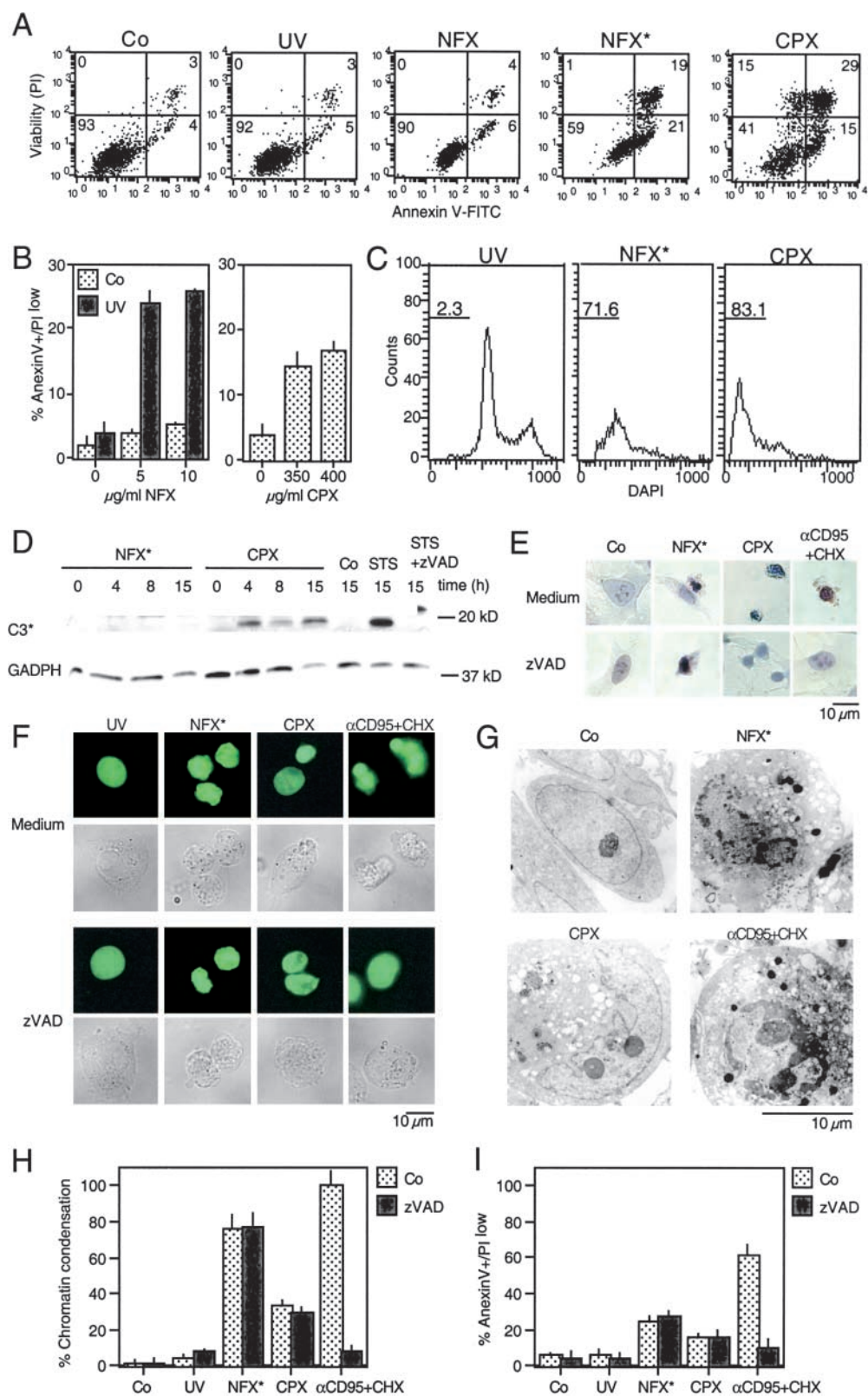
Figure 2. Caspase-independent cell death induction by NFX* and CPX. (A) PS exposure resulting from lysosomal destabilization. After the indicated treatment, cells were stained for PS exposure (with annexin V-FITC) or plasma membrane permeabilization (with PI) and subjected to cytofluorometric analysis. Numbers in each quadrant refer to the percentage of cells. (B) Quantitation of data obtained in A. (C) DNA hypodiploidy induced by NFX* and CPX. After 24 h, the nuclear DNA content was determined with DAPI by cytofluorometric analysis in fixed-permeabilized cells. Numbers indicate the percentage of cells exhibiting a subdiploid (apoptotic) DNA content. (D) Immunoblot determination of caspase-3 maturation. Cell extracts obtained after the indicated treatment and interval were subjected to immunoblotting with antibodies specific for cleaved caspase-3 (17-kD fragment) and glyceraldehyde-3-phosphate dehydrogenase (as a loading control). (E) Giemsa staining of HeLa cells treated with NFX*, CPX, or αCD95, in the absence or presence of 100 μM z-VAD-fmk. (F) Chromatin structure of living HeLa cells stably expressing a histone H2B-GFP fusion protein after treatment with NFX* or CPX. Representative micrographs of the GFP fluorescence and phase-contrast pictures are shown. (G) Ultrastructure of NFX*- or CPX-treated cells exhibiting nuclear chromatin condensation and vacuolization, as compared with apoptosis induced by αCD95. (H) Chromatin condensation induced by NFX* or CPX, both in the absence or presence of 100 μM z-VAD-fmk, as determined in F. (I) Failure of z-VAD-fmk (100 μM) to inhibit PS exposure in NFX*- and CPX-treated cells. Data are shown as mean values ± SD of three independent experiments.
