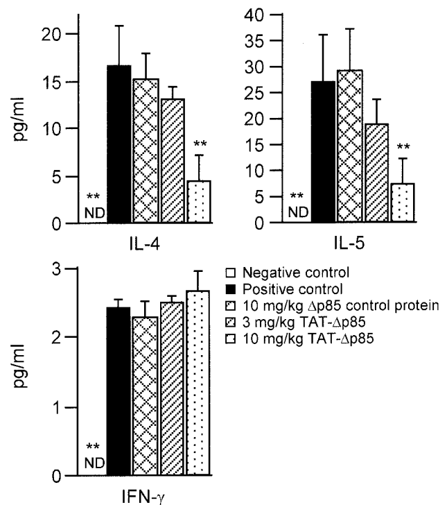
Figure 6. Effect of TAT- \Delta p85 on Th1 and Th2 cytokine secretion after four OVA challenges on days 21, 22, 23, and 24. BAL fluids were collected 24 h after the last OVA challenge. Positive (■) and negative (□) controls are OVA and saline challenged animals, respectively, without any pretreatment. TAT- \Delta p85 reduces the level of Th2 cytokines, IL-4 and IL-5, but has no effect on the Th1 cytokine IFN \gamma . Note difference in scale on the ordinate. Each bar represents the mean \pm SEM of 4–6 mice. ** P < 0.01 compared with positive control group. ND, not detectable.
