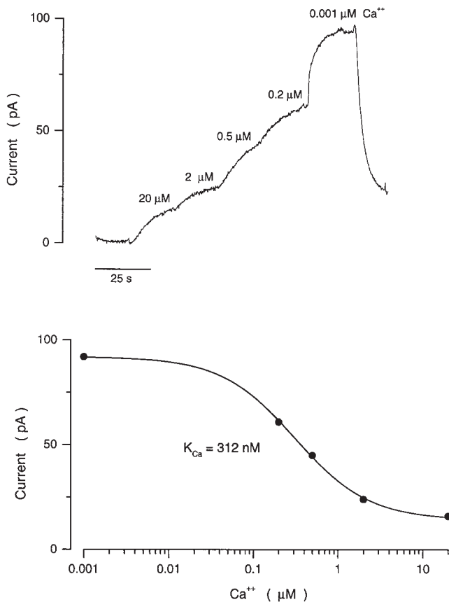
FIGURE 5. \text{Ca}^{2+} dependence of the 8Br-cGMP-activated current in an electropermeabilized single cone. The cell was electropermeabilized in the presence of 20 \mu\text{M} \text{Ca}^{2+} without \text{Mg}^{2+} , current was then activated with 40 \mu\text{M} 8Br-cGMP and the free concentration of \text{Ca}^{2+} was progressively reduced in steps to 1 \text{ nM} . (top) Currents measured with this experimental protocol. We consistently observed that the response time constant to changes in \text{Ca}^{2+} concentration was slower than that to changes in cyclic nucleotide concentration. (bottom) The dependence of current amplitude on \text{Ca}^{2+} concentration. The continuous curve illustrates an optimum fit to the experimental data of the inverse Hill function (Eq. 2). For the data shown, K_{\text{Ca}} = 312 \text{ nM} and n = 1.4 .
