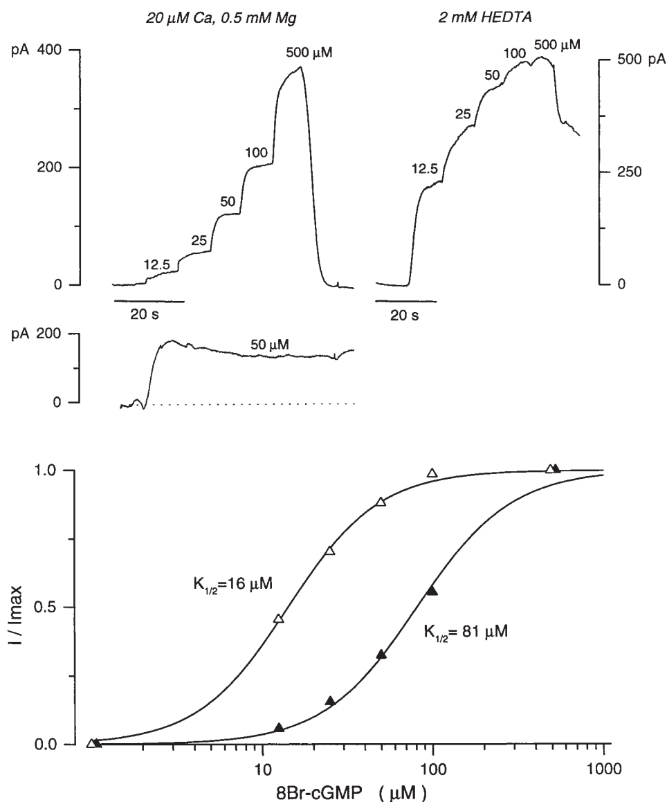
FIGURE 3. \text{Ca}^{2+} -dependent modulation of activation by 8Br-cGMP of the cyclic nucleotide-gated channels in electroporabilized striped bass single cones. (top left) Outer segment currents measured in the presence of 20 \mu\text{M Ca}^{2+} and 0.5 \text{ mM Mg}^{2+} in response to increasing nucleotide concentrations. Also shown is the continuous response of a different ep-cone to a single step of subsaturating 8Br-cGMP ( 50 \mu\text{M} ). The example shown is atypical, but was selected to illustrate extreme drift in current amplitude and make evident its small contribution to experimental error in the determination of the values of K_{1/2} and n in the Hill equation (Eq. 1). (top right) Currents activated by 8Br-cGMP in the absence of divalent cations. (bottom) The continuous curves illustrate the Hill equation that best fits the experimental data. For the data shown, K_{1/2} = 81 \mu\text{M cGMP} and n = 1.3 in the presence of divalent cations ( \blacktriangle ), and K_{1/2} = 16 \mu\text{M cGMP} and n = 1.1 in their absence ( \triangle ).
