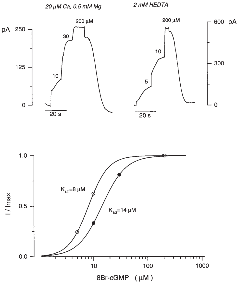
FIGURE 4. \text{Ca}^{2+} -dependent modulation of activation by 8Br-cGMP of the cGMP-gated channels in electropermeabilized tiger salamander rods. ( top left ) Outer segment currents measured in the presence of 20 \mu\text{M} \text{Ca}^{2+} and 0.5 \text{ mM} \text{Mg}^{2+} in response to increasing nucleotide concentrations. ( top right ) Currents activated by 8Br-cGMP in the absence of divalent cations. ( bottom ) The continuous curves illustrate the Hill equation that best fits the experimental data. For the data shown, K_{1/2} = 14 \mu\text{M} cGMP and n = 2 in the presence of divalent cations (●), and K_{1/2} = 8 \mu\text{M} cGMP and n = 2.3 in their absence (○).
