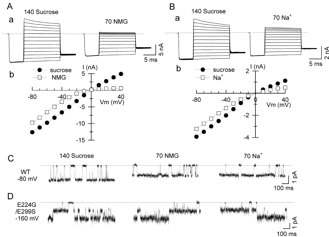
FIGURE 5. Effects of ionic strength on wild-type and mutant Kir2.1 channel currents. Ionic strength was increased by replacing 140 mM sucrose with 70 mM NMG + or 70mM Na + . (A and B) Macroscopic currents (a) of wild-type Kir2.1 channel were recorded with symmetrical 30 mM K in intracellular and extracellular solutions. The macroscopic I-V curves in the presence of sucrose vs. NMG + or Na + are shown in (b) in both panels. (C) Single channel recording from wild-type Kir2.1 under symmetrical 30 mM K + conditions at holding potential of -80 mV. (D) Single channel recording of the double mutant channel E224G/E299S under the same condition at holding potential of -160 mV. There were two channels in this patch.
